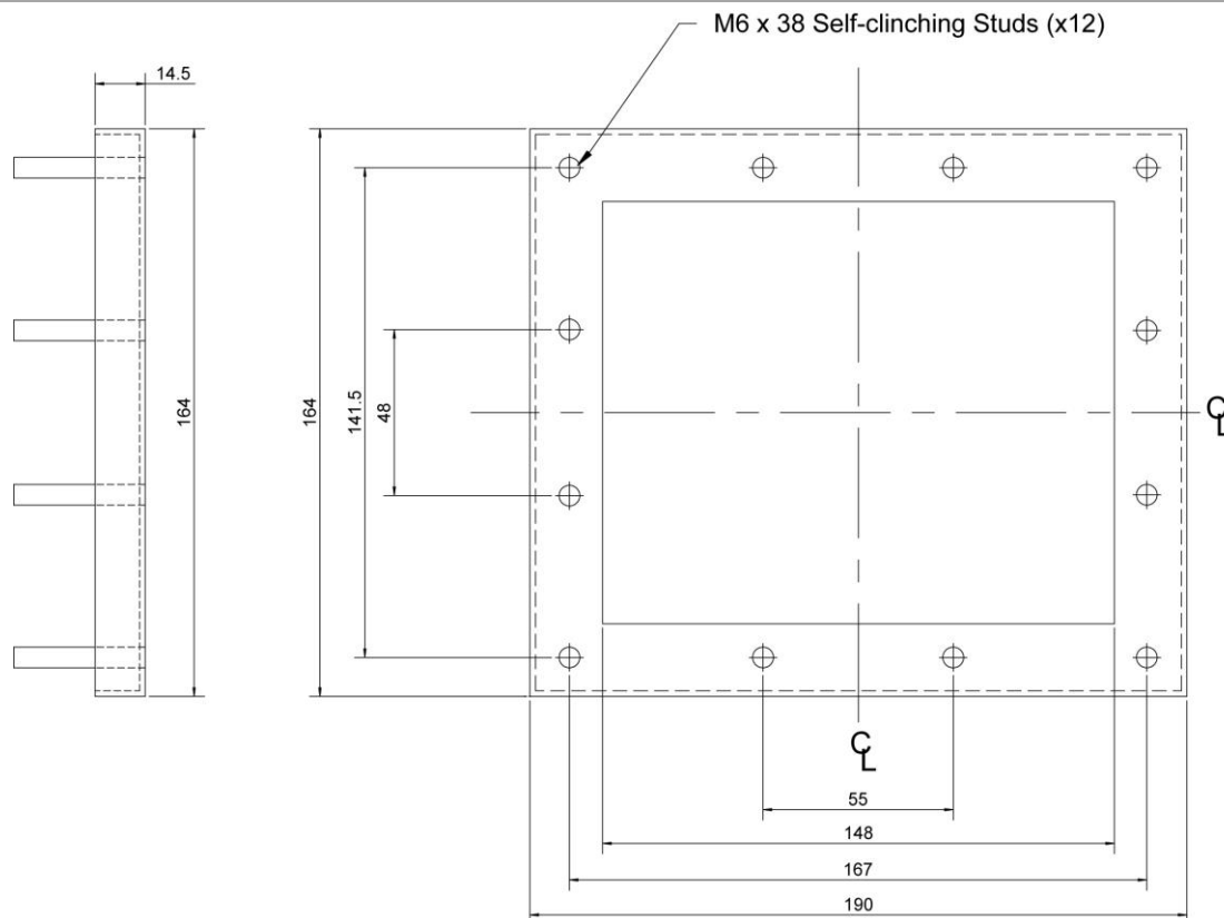
Figure 1: Dimensions of Omni8C IP65 Cover [Omni8C cut-out dimensions: 112mm (4.41") x 136mm (5.35")]
