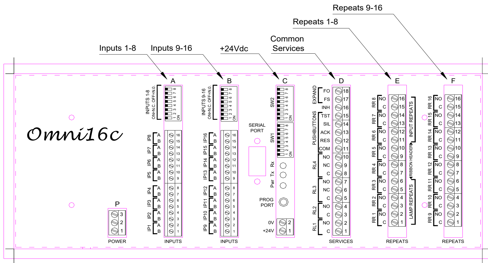
Figure 2-4 – Omni16C Rear View
