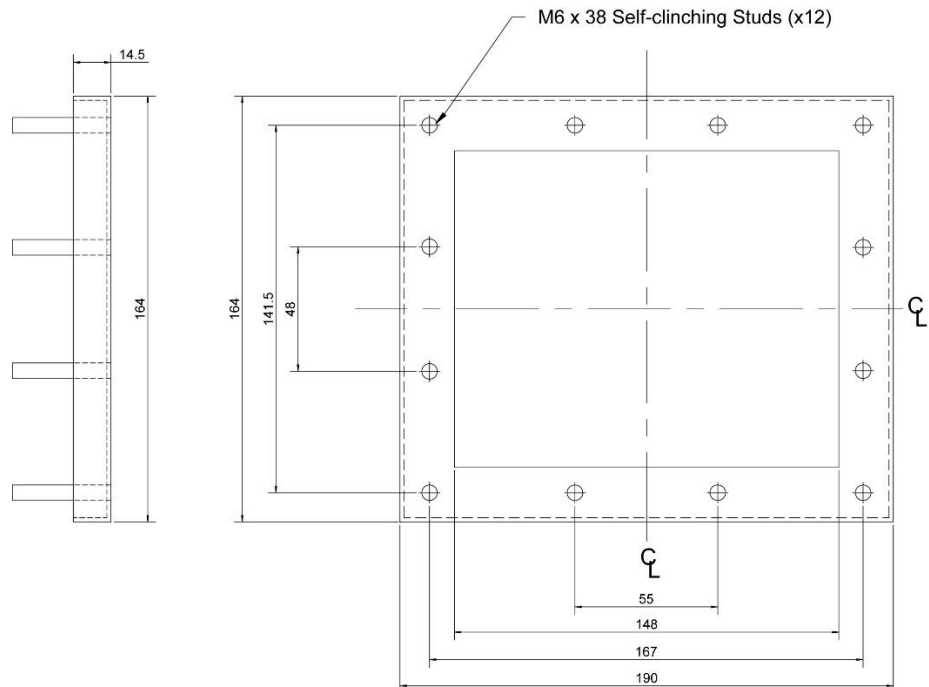
Figure 3-9 – Omni8 IP65 Front Cover Mechanical Mounting.
