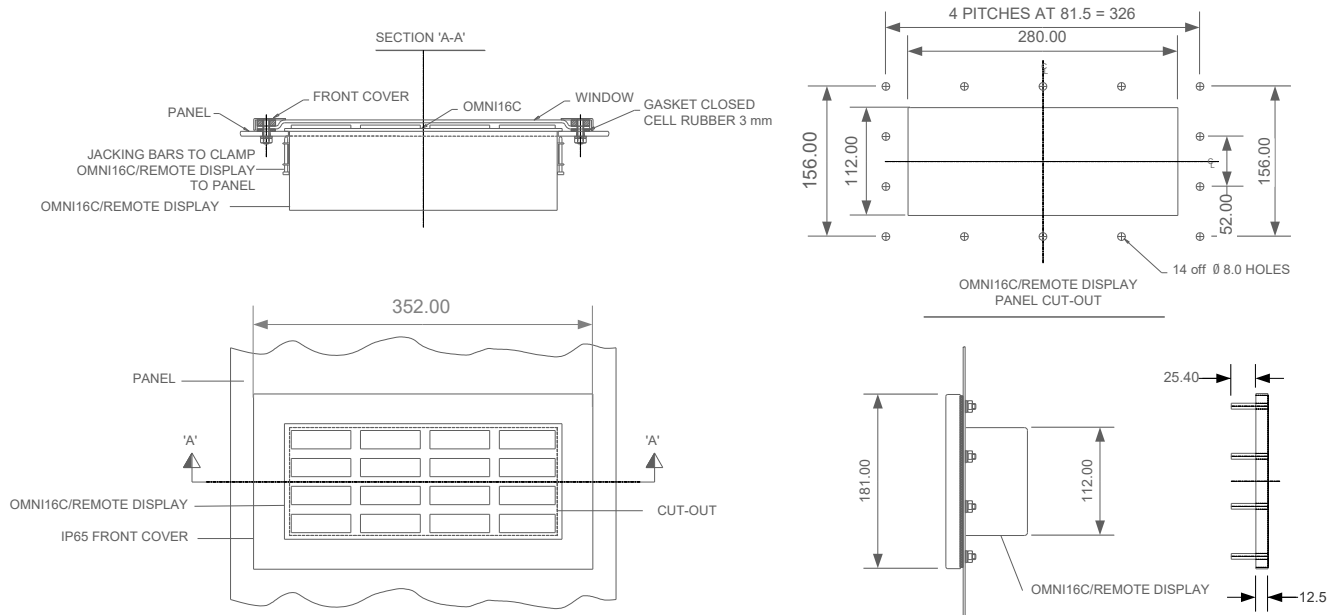
Figure 3-8 – Omni16C IP65 Front Cover Mechanical Mounting.
