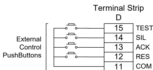
Figure 4-10 – External Pushbuttons controlling a single Omni8/16C
